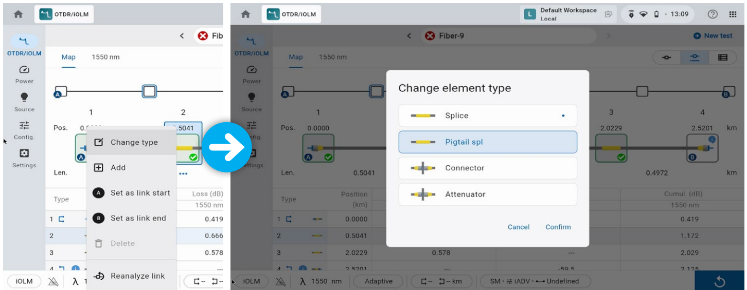
When you change events from a regular connector (threshold at 0.5 db in the example above) to a custom "pigtail spliced connector," a custom-built icon appears and the unit adjusts to a custom threshold (0.75 db in the example above) so you can avoid false failures. Modified elements are tagged with an asterisk (*) for traceability.
